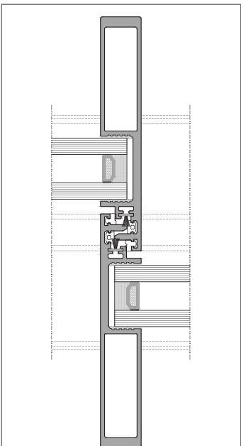
Interlock Section
