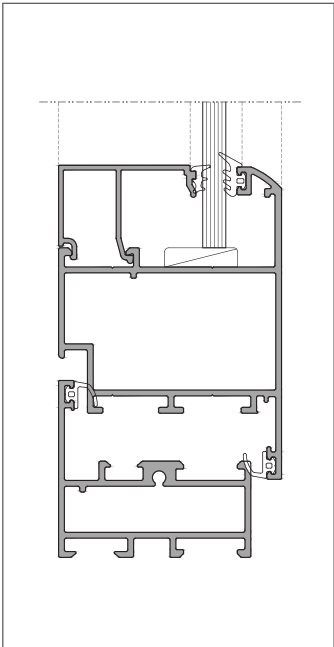
Bottom Section
