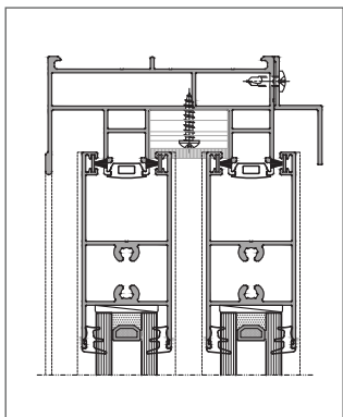
Top Section
