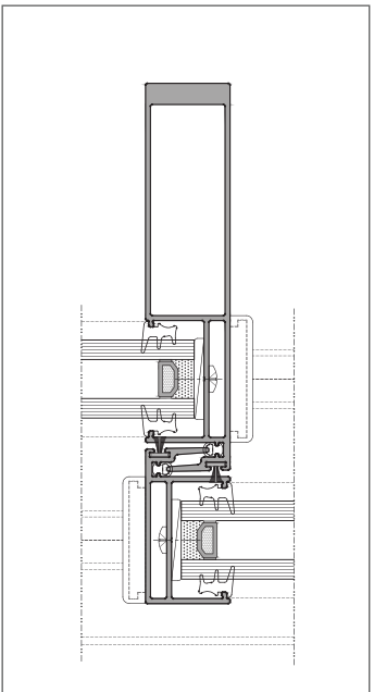
Interlock Section
