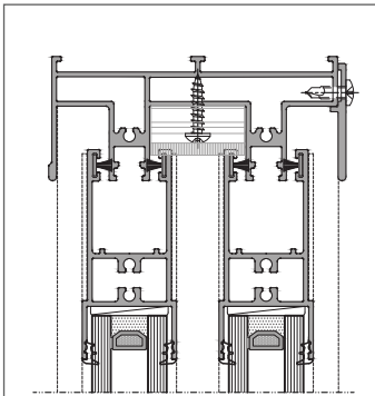
Top Section
