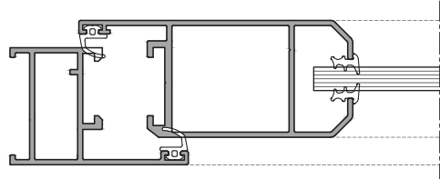
Handle Section
