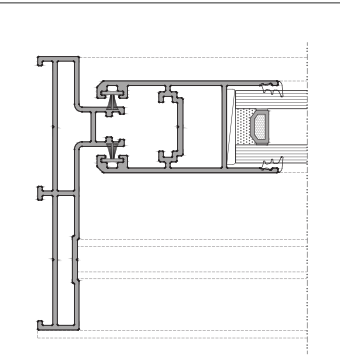
Handle Section
