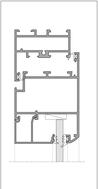
Top Section
