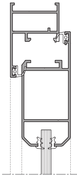
Top Section
