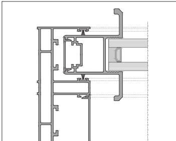
Handle Section
