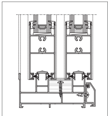
Bottom Section
