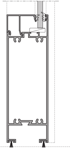
Bottom Section
