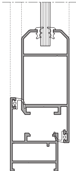
Bottom Section
