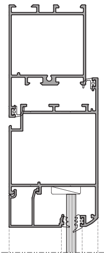
Top Section
