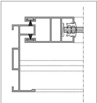
Handle Section
