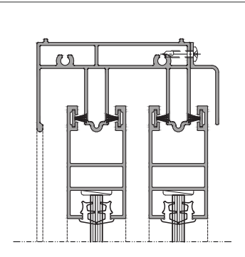
Top Section
