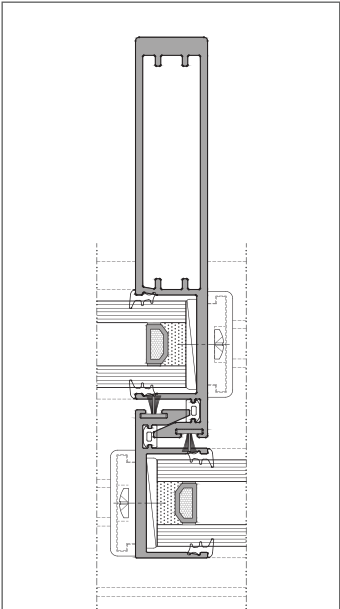
Interlock Section
