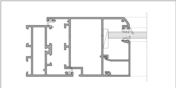
Handle Section
