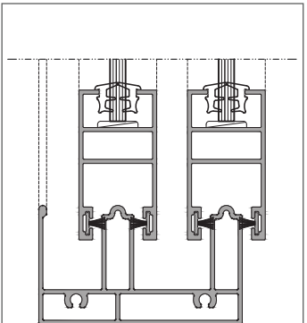
Bottom Section
