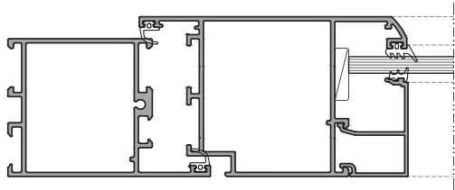
Handle Section
