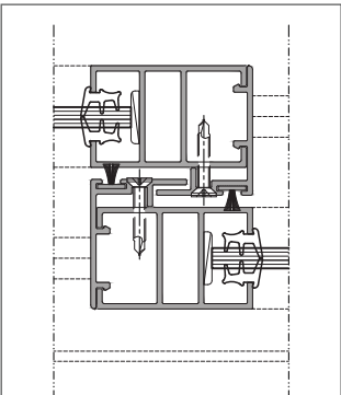
Interlock Section
