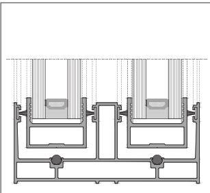
Bottom Section
